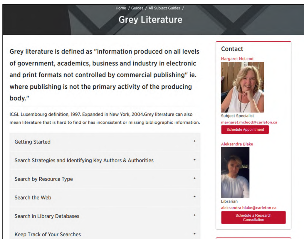
Figure 2: Webpage
