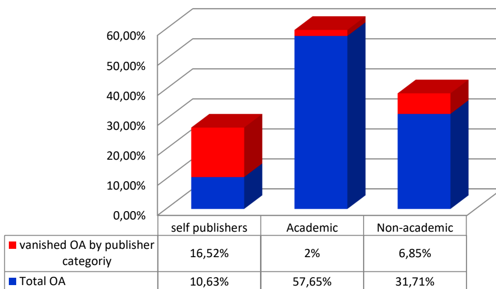
Figure 3 - Number of vanished OA by publishers category
