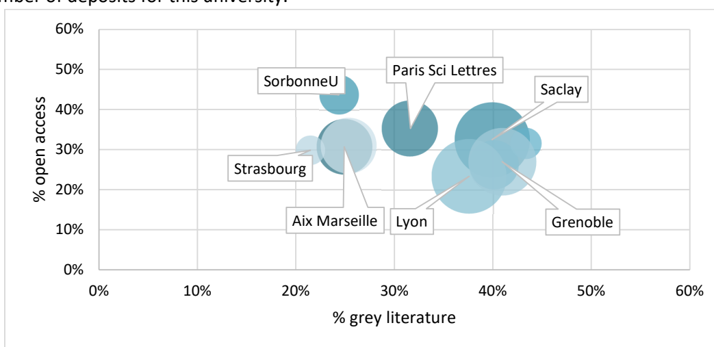
Figure 7. Degree of openness and part of grey literature per university (N=973,968 deposits)
